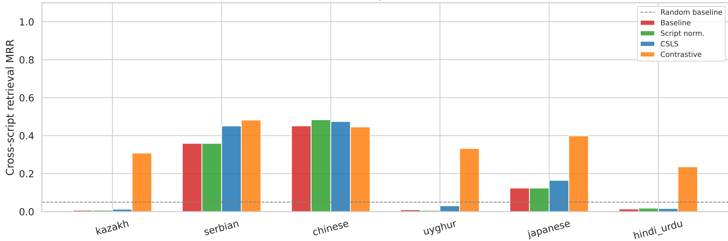
Experiment 6: Cross-script retrieval MRR under four conditions (XLM-R, final layer unless noted)
